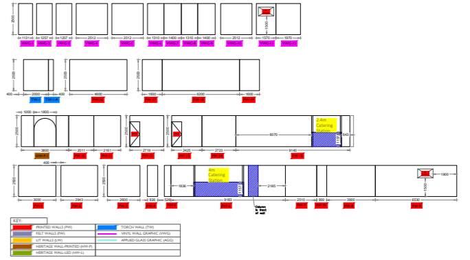
LE 98 Wall Elevations
